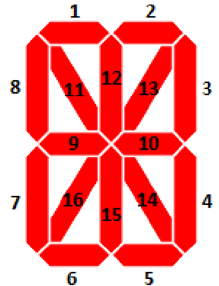
16-segment display
