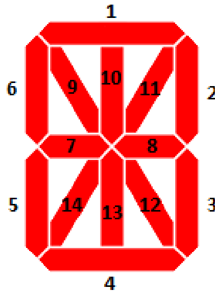
14-segment display
