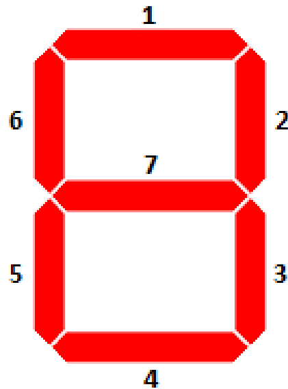
7-segment display
